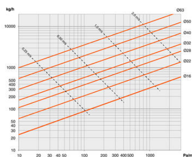
Pressure loss sanitary PN10
